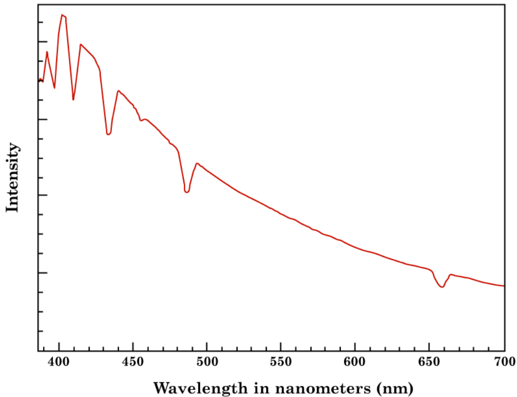
Visible Spectrum — Vega
