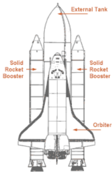
Space Shuttle (launch configuration)
